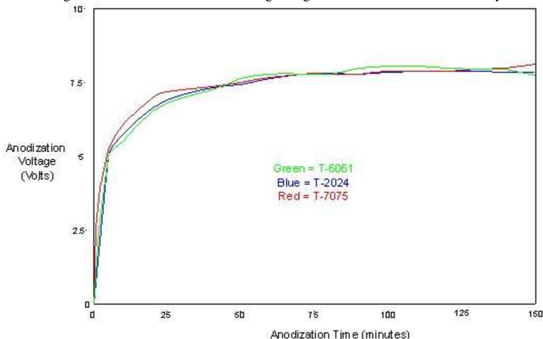
Figure 1. shows the measured anodizing voltage of three common aluminum alloys over time.
