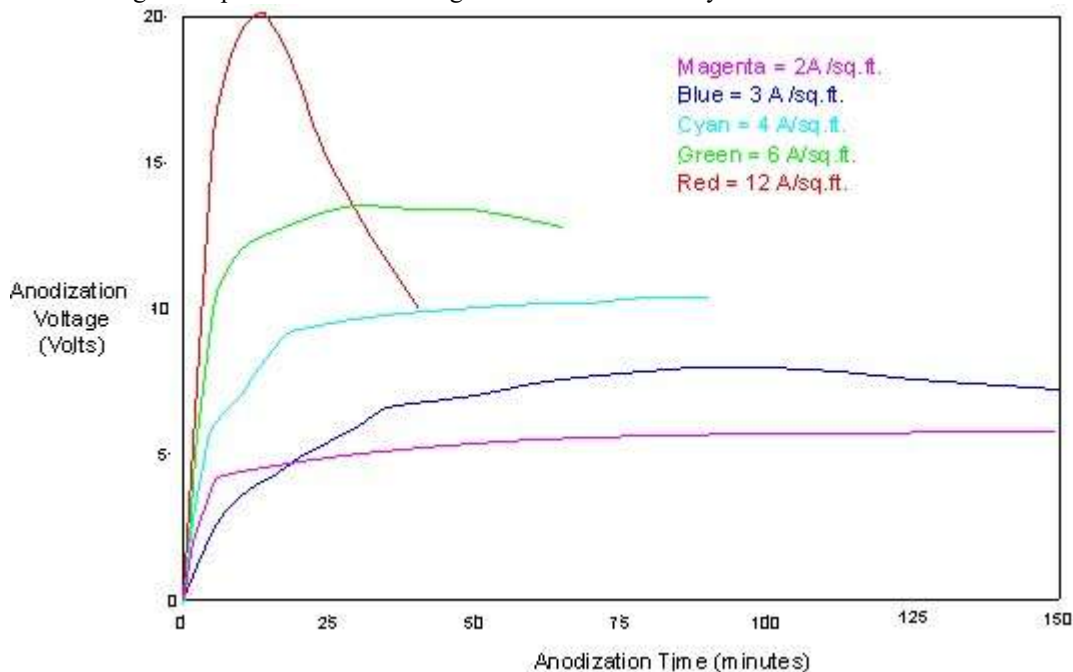
2. Anodizing Curves for various Current Densities
